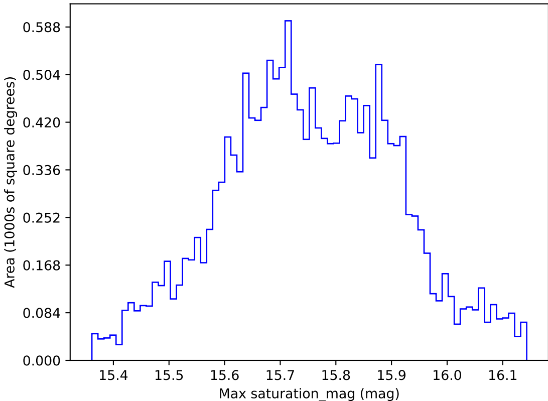
too_elab_r32_d2_gz_v3.4_10yrs WFD r band: Max saturation_mag
