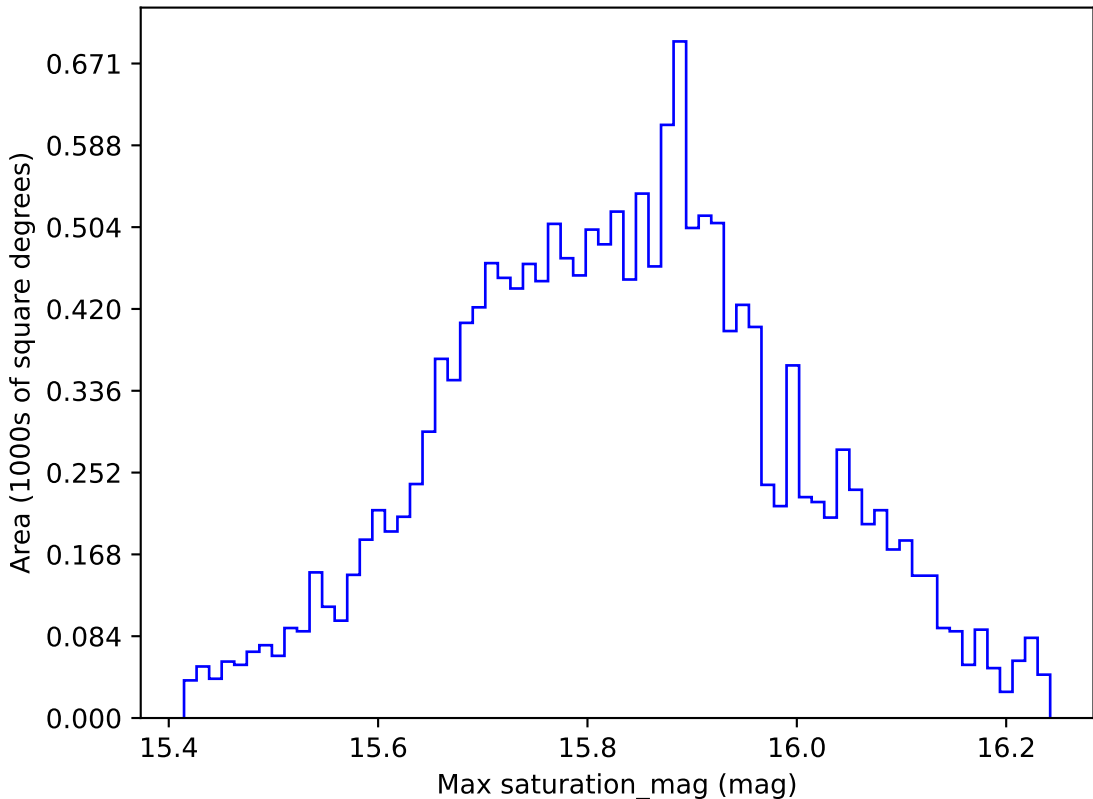
too_elab_r32_d2_gz_v3.4_10yrs WFD all bands: Max saturation_mag
