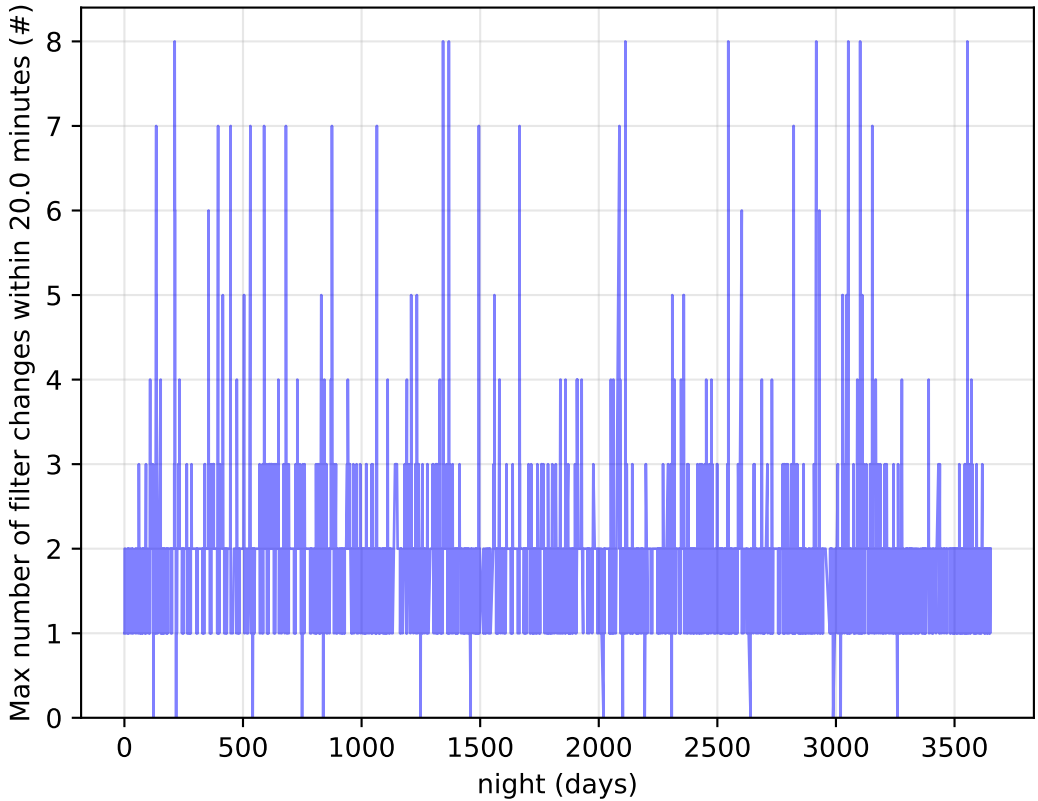
too_elab_r32_d2_gz_v3.4_10yrs Per Night: Max number of filter changes within 20.0 minutes
