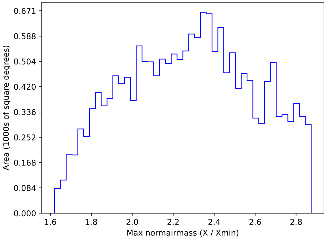
too_elab_r32_d2_gz_v3.4_10yrs WFD z band: Max normairmass
