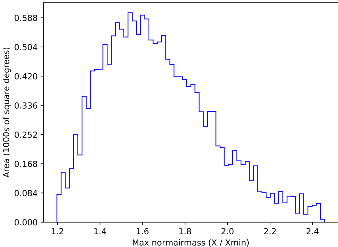
too_elab_r32_d2_gz_v3.4_10yrs WFD u band: Max normairmass
