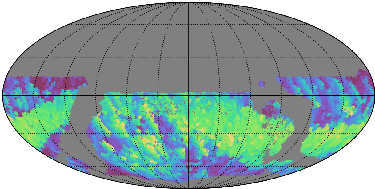
too_elab_r32_d2_gz_v3.4_10yrs WFD r band: Max normairmass
