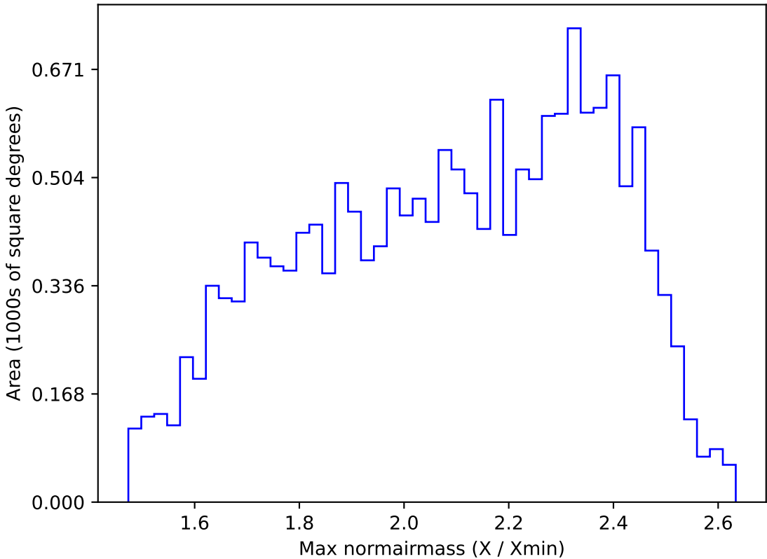
too_elab_r32_d2_gz_v3.4_10yrs WFD r band: Max normairmass
