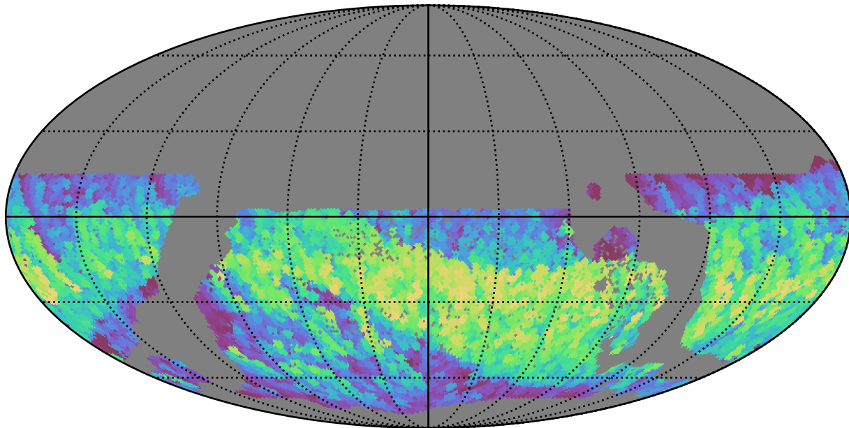
too_elab_r32_d2_gz_v3.4_10yrs WFD i band: Max normairmass
