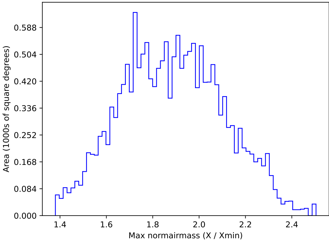
too_elab_r32_d2_gz_v3.4_10yrs WFD g band: Max normairmass
