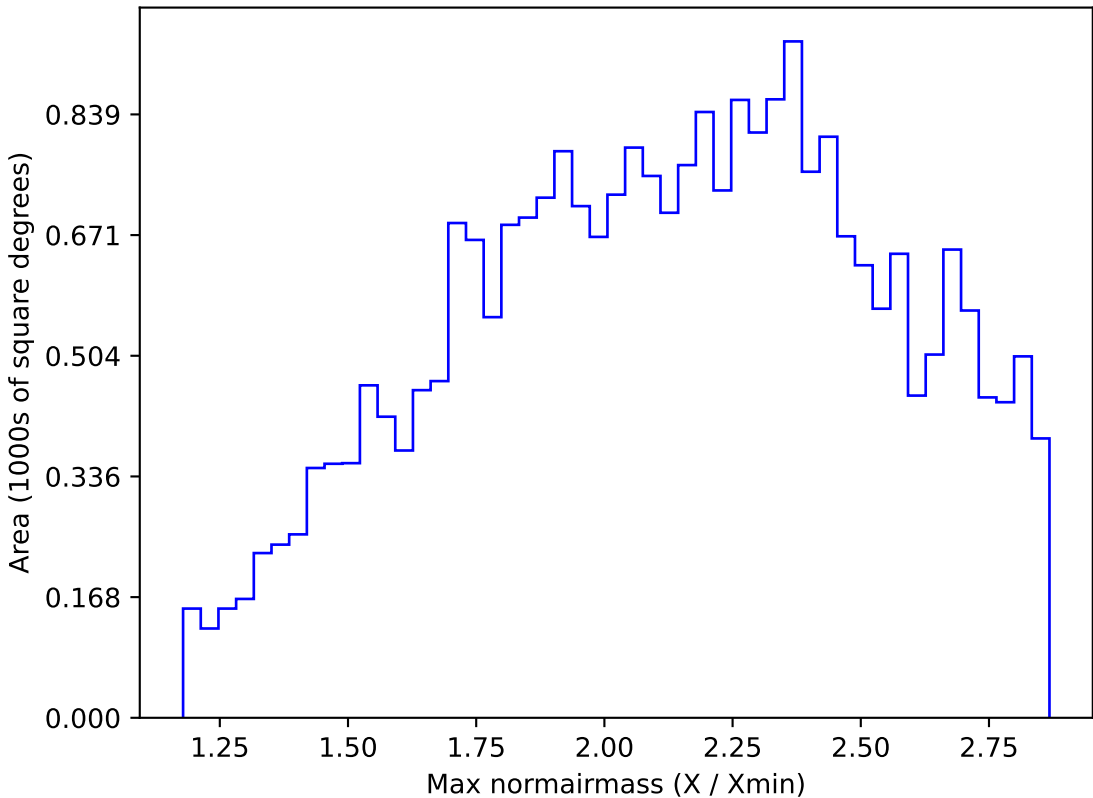
too_elab_r32_d2_gz_v3.4_10yrs All sky z band: Max normairmass
