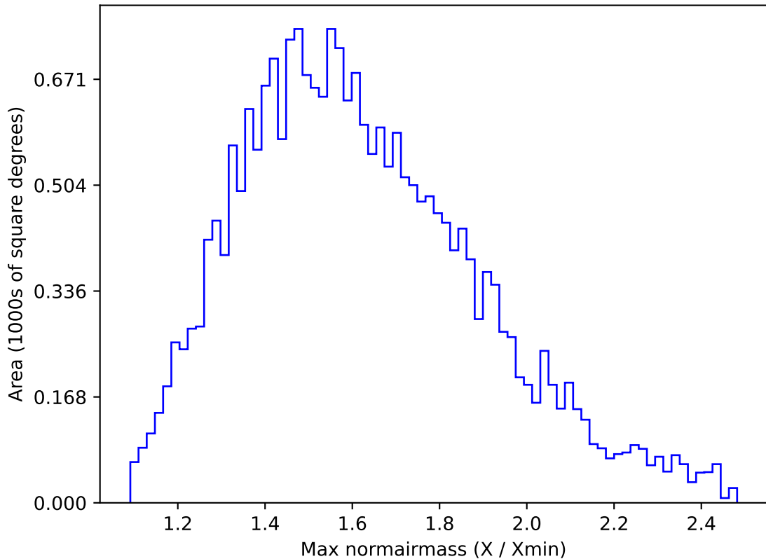
too_elab_r32_d2_gz_v3.4_10yrs All sky u band: Max normairmass
