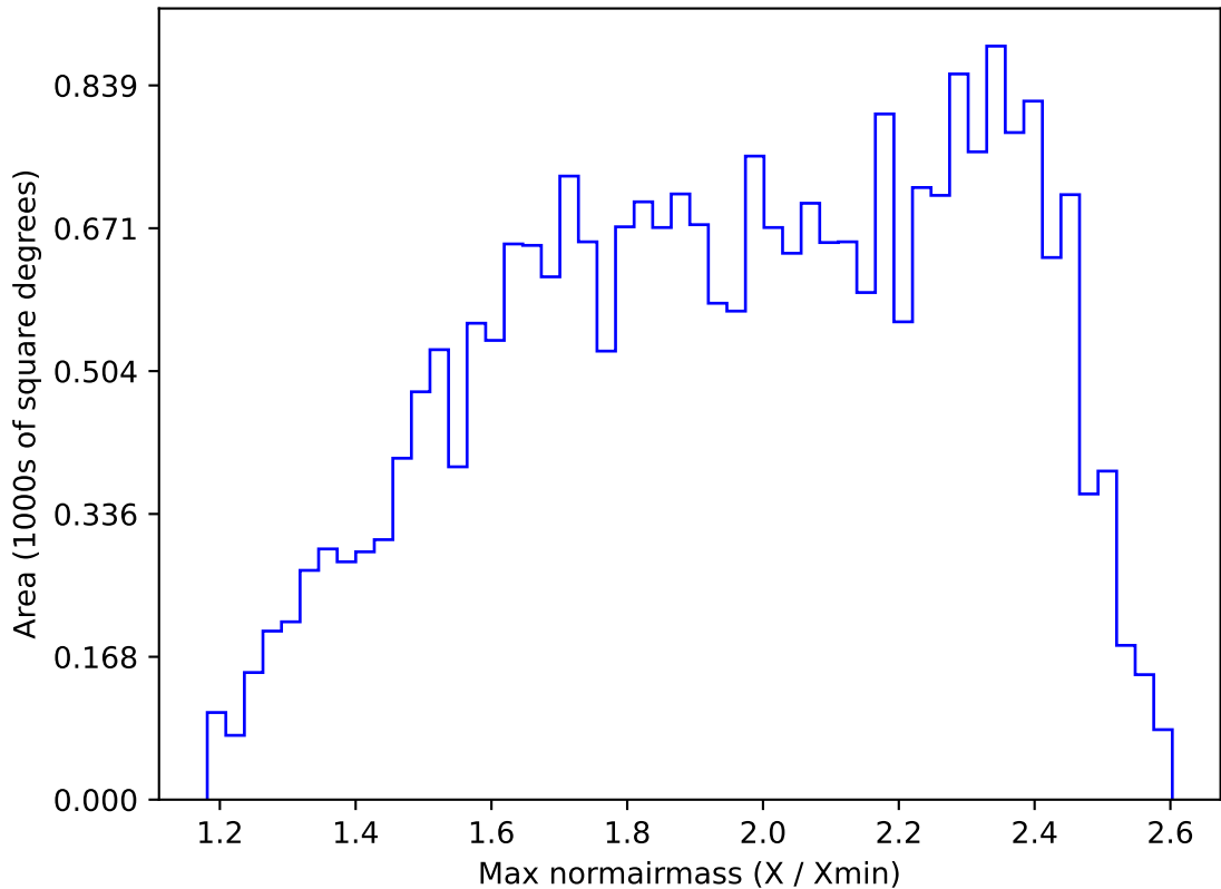
too_elab_r32_d2_gz_v3.4_10yrs All sky r band: Max normairmass
