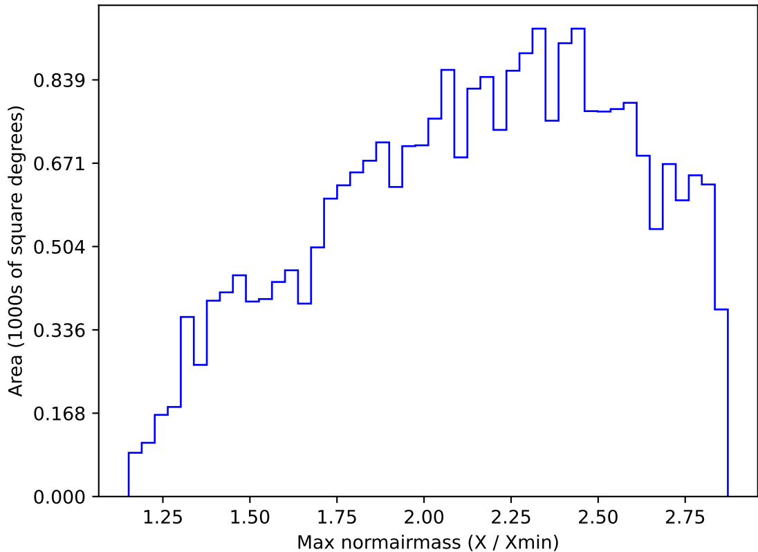
too_elab_r32_d2_gz_v3.4_10yrs All sky i band: Max normairmass
