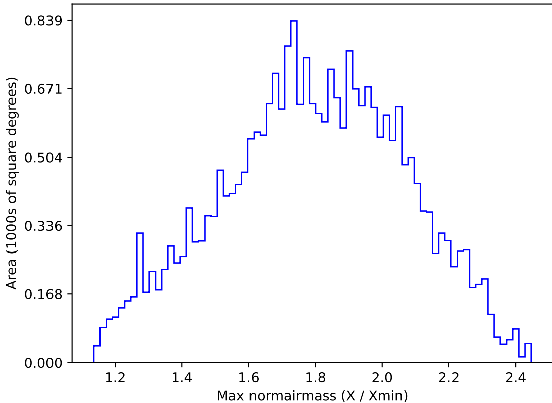
too_elab_r32_d2_gz_v3.4_10yrs All sky g band: Max normairmass
