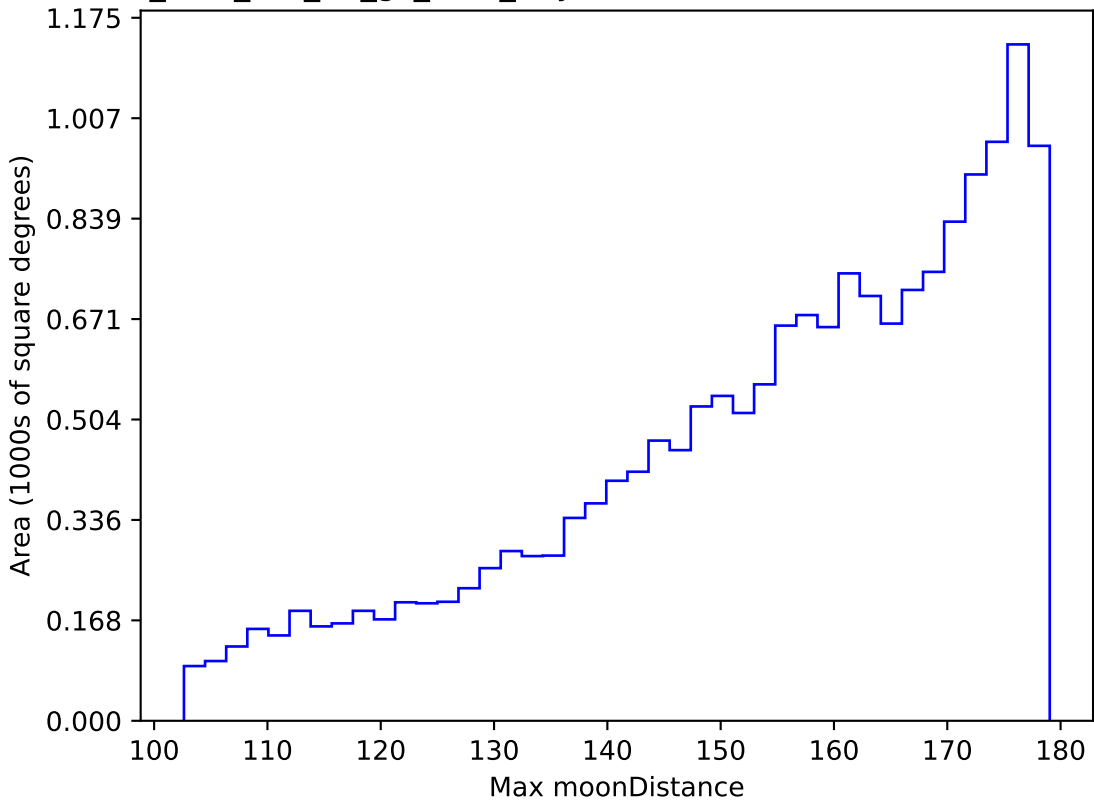
too_elab_r32_d2_gz_v3.4_10yrs WFD z band: Max moonDistance
