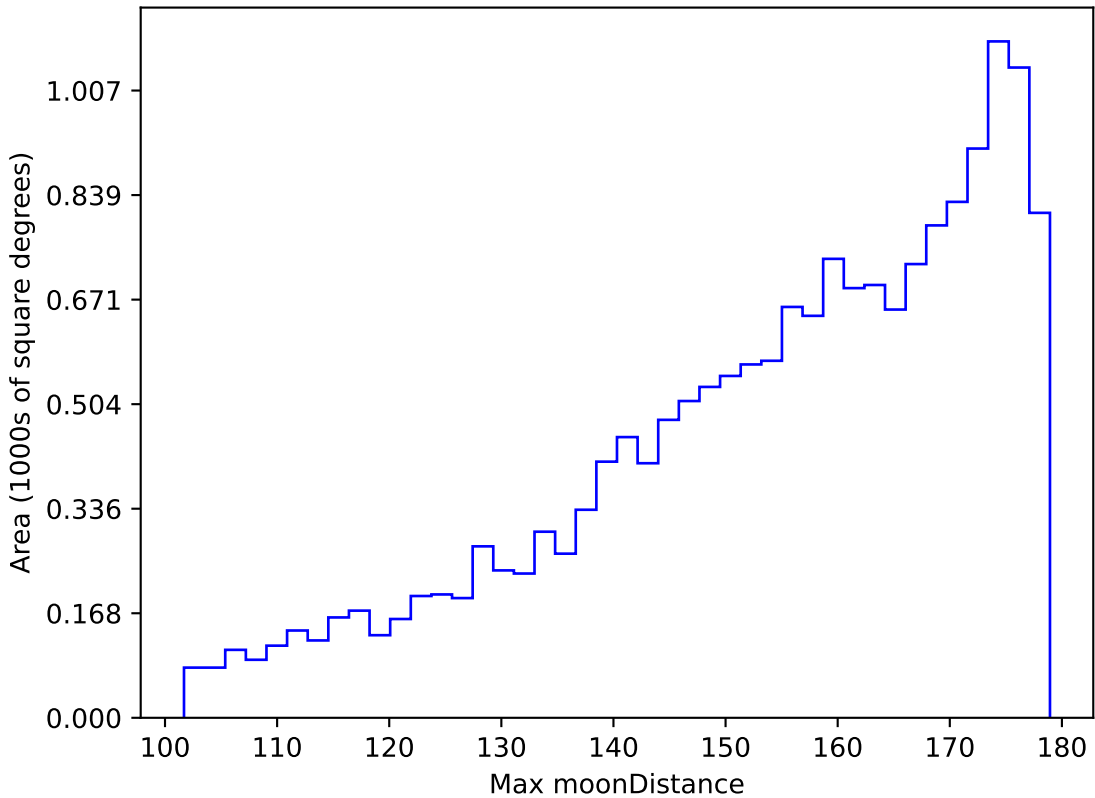
too_elab_r32_d2_gz_v3.4_10yrs WFD u band: Max moonDistance
