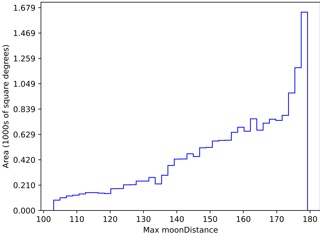
too_elab_r32_d2_gz_v3.4_10yrs WFD r band: Max moonDistance
