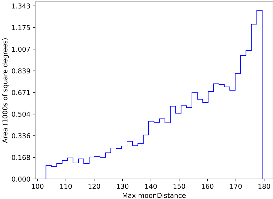
too_elab_r32_d2_gz_v3.4_10yrs WFD i band: Max moonDistance
