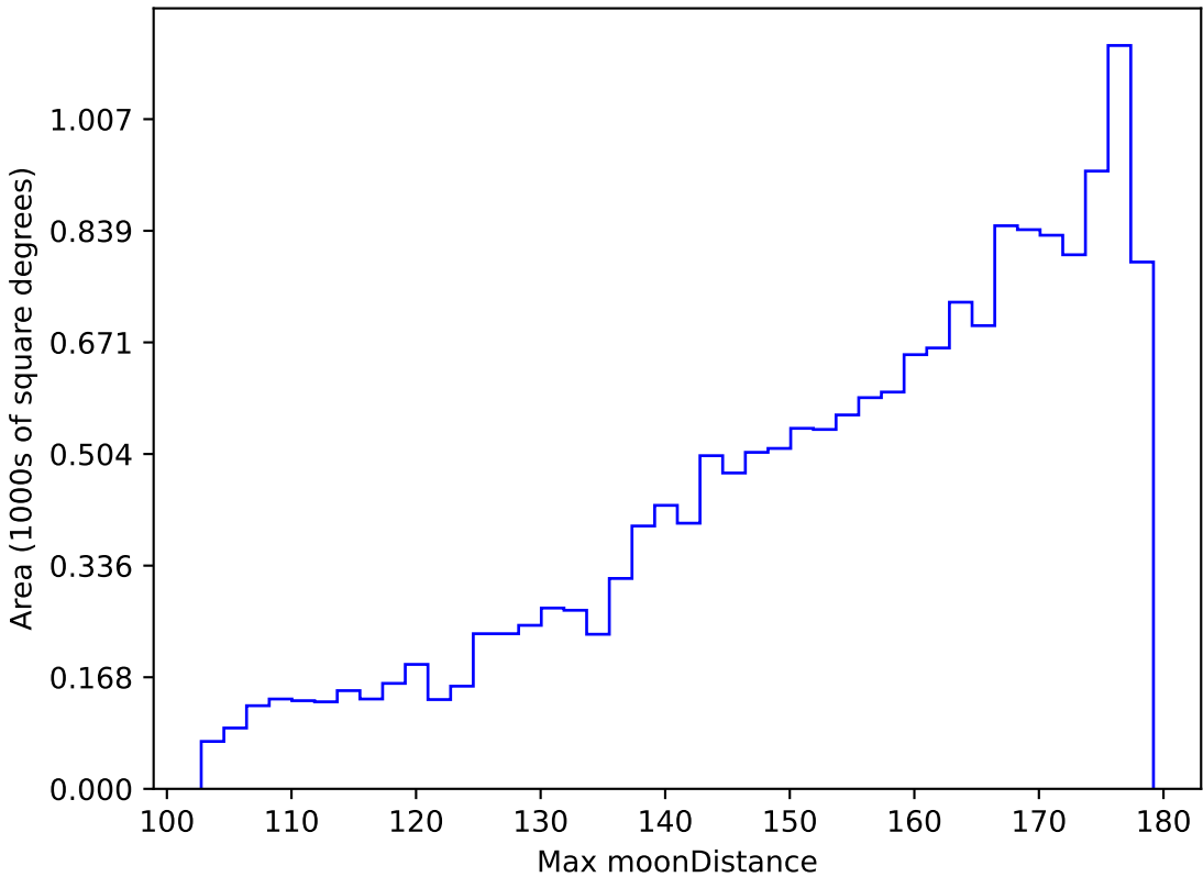
too_elab_r32_d2_gz_v3.4_10yrs WFD g band: Max moonDistance
