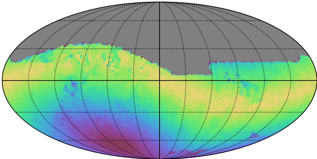
too_elab_r32_d2_gz_v3.4_10yrs All sky z band: Max moonDistance
