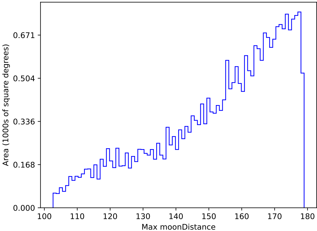
too_elab_r32_d2_gz_v3.4_10yrs All sky z band: Max moonDistance
