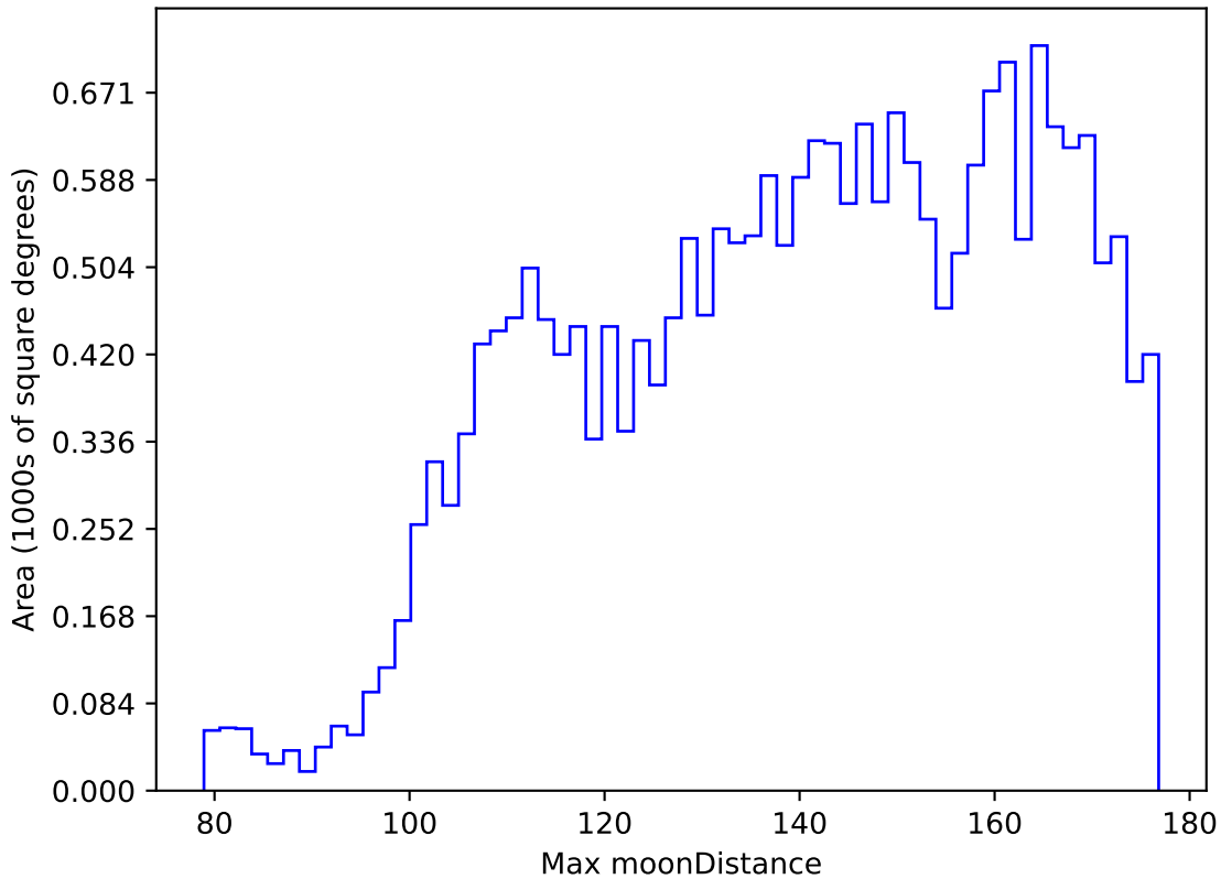
too_elab_r32_d2_gz_v3.4_10yrs All sky y band: Max moonDistance
