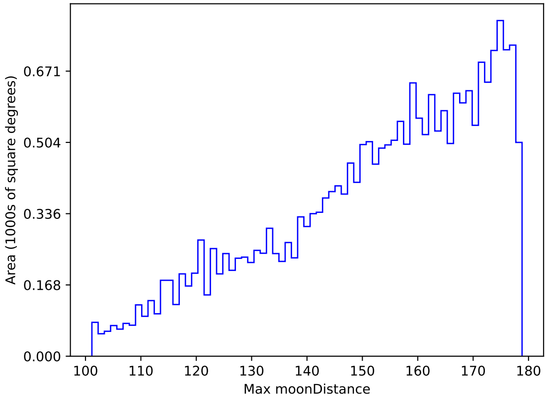
too_elab_r32_d2_gz_v3.4_10yrs All sky u band: Max moonDistance
