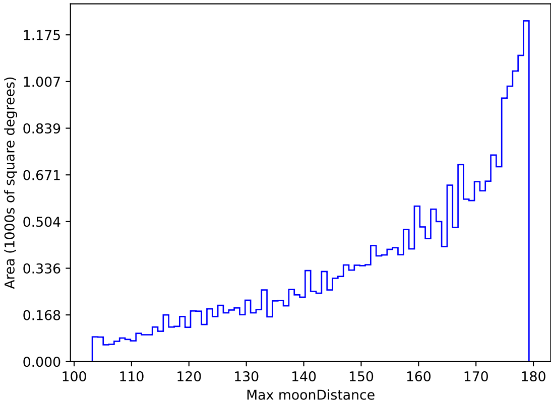
too_elab_r32_d2_gz_v3.4_10yrs All sky r band: Max moonDistance
