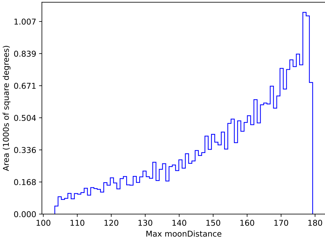
too_elab_r32_d2_gz_v3.4_10yrs All sky i band: Max moonDistance
