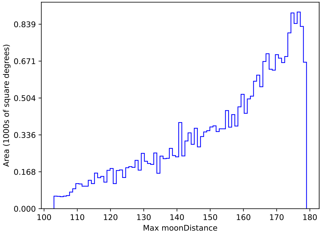
too_elab_r32_d2_gz_v3.4_10yrs All sky g band: Max moonDistance
