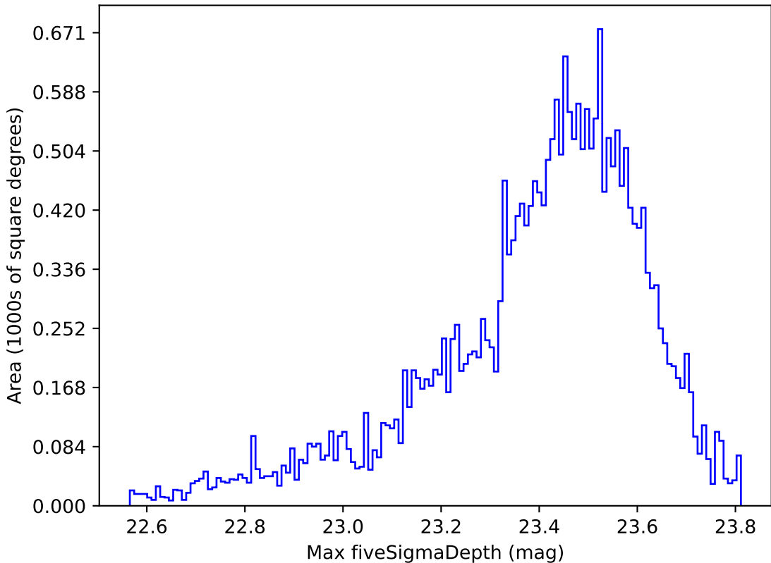
too_elab_r32_d2_gz_v3.4_10yrs Yr 1 z band: Max fiveSigmaDepth
