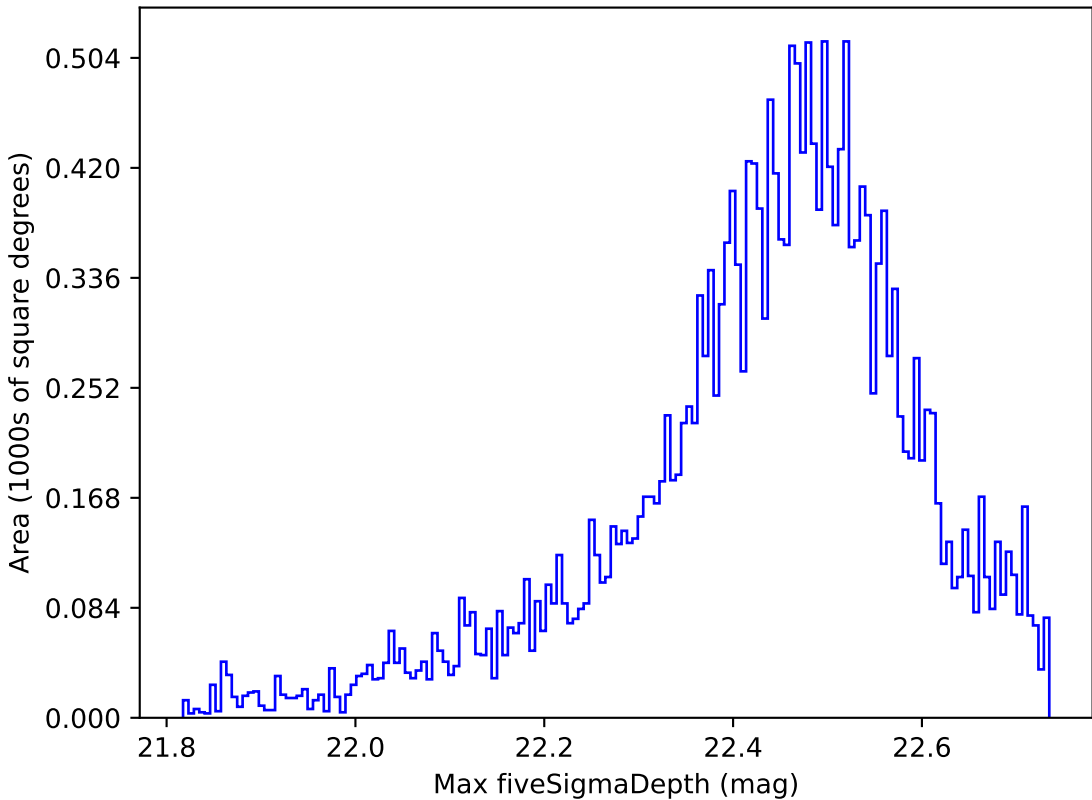
too_elab_r32_d2_gz_v3.4_10yrs Yr 1 y band: Max fiveSigmaDepth
