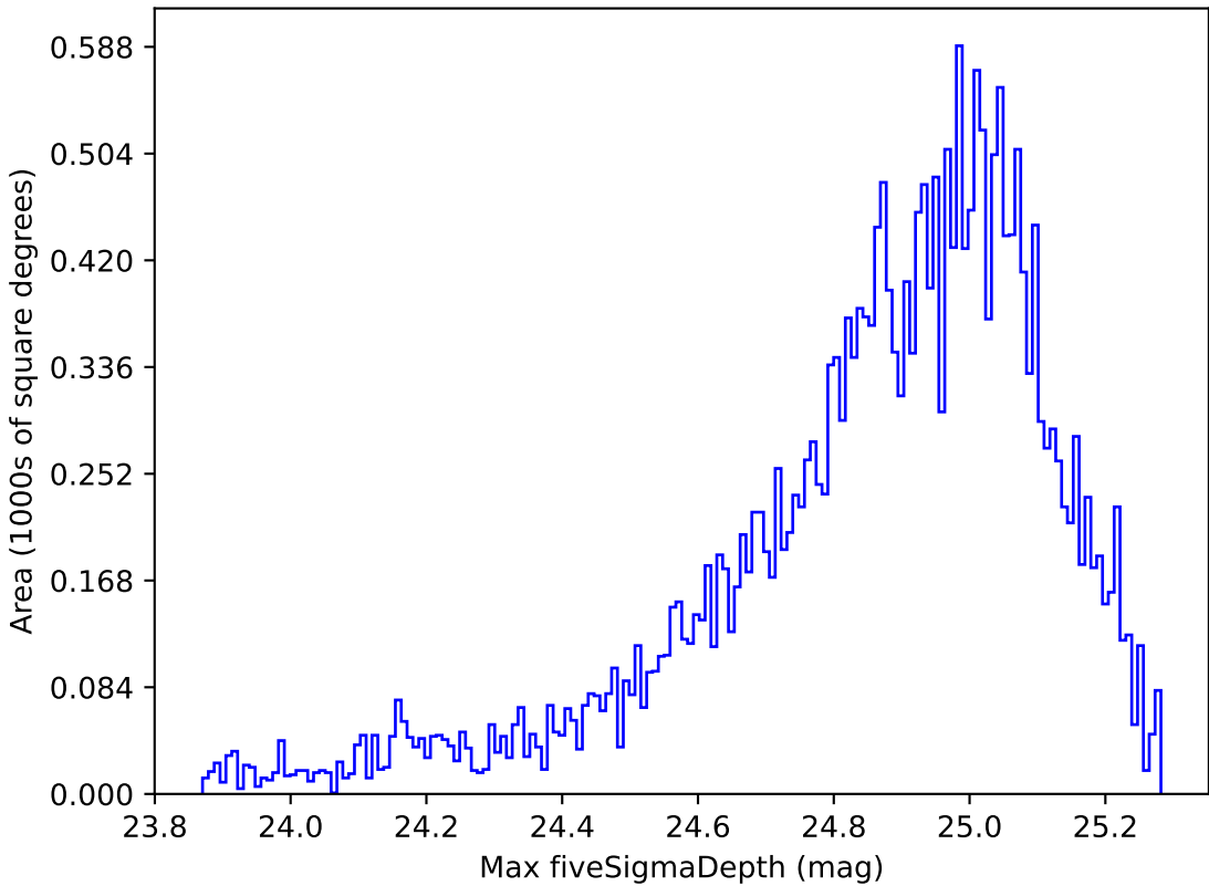
too_elab_r32_d2_gz_v3.4_10yrs Yr 1 g band: Max fiveSigmaDepth
