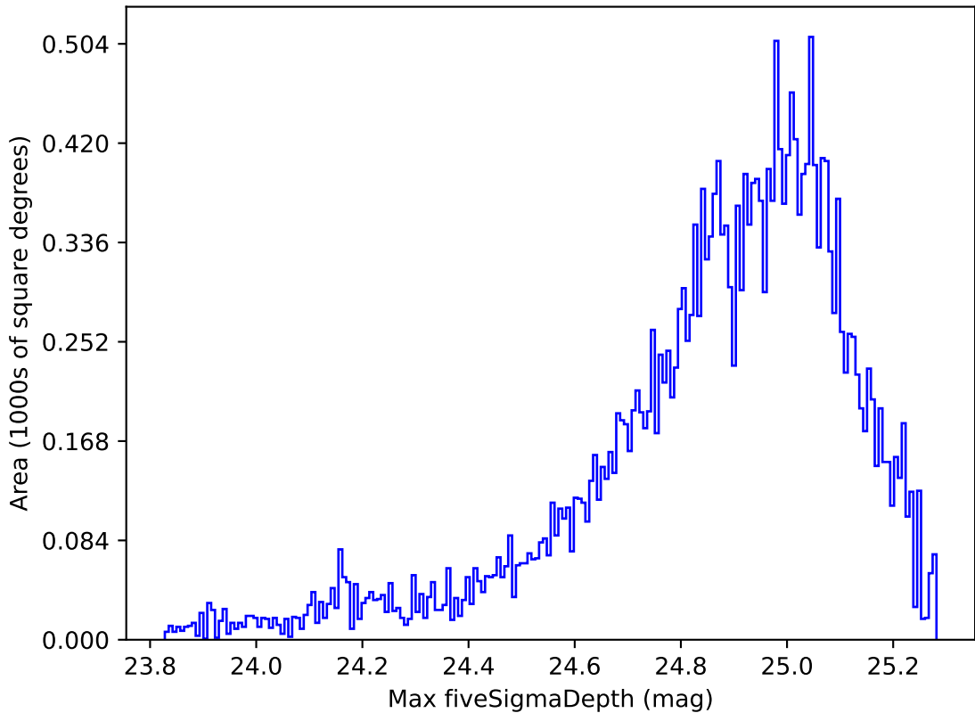
too_elab_r32_d2_gz_v3.4_10yrs Yr 1 all bands: Max fiveSigmaDepth
