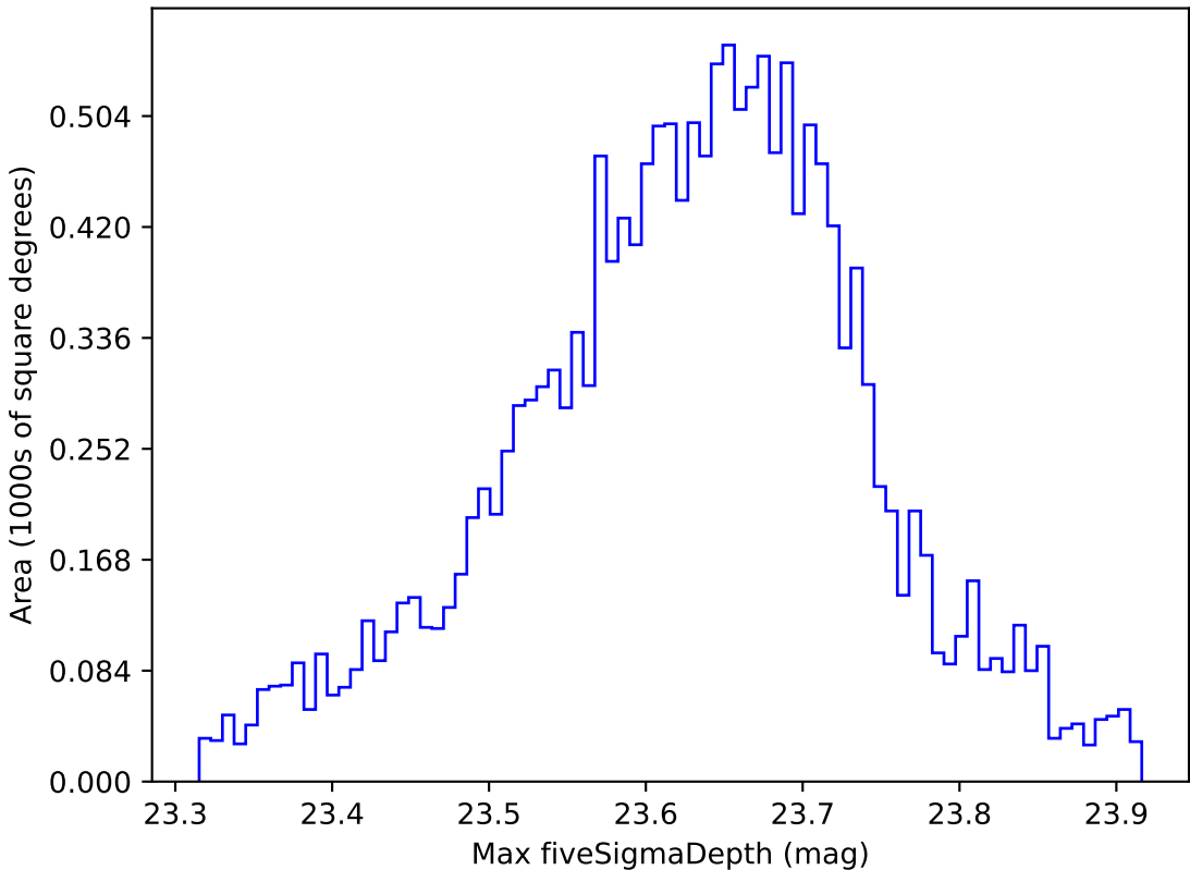
too_elab_r32_d2_gz_v3.4_10yrs WFD z band: Max fiveSigmaDepth
