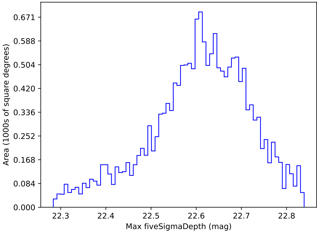
too_elab_r32_d2_gz_v3.4_10yrs WFD y band: Max fiveSigmaDepth
