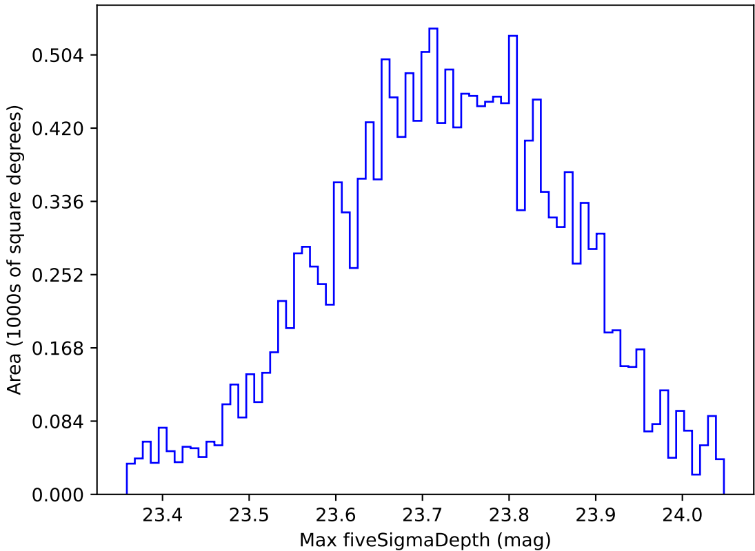
too_elab_r32_d2_gz_v3.4_10yrs WFD u band: Max fiveSigmaDepth
