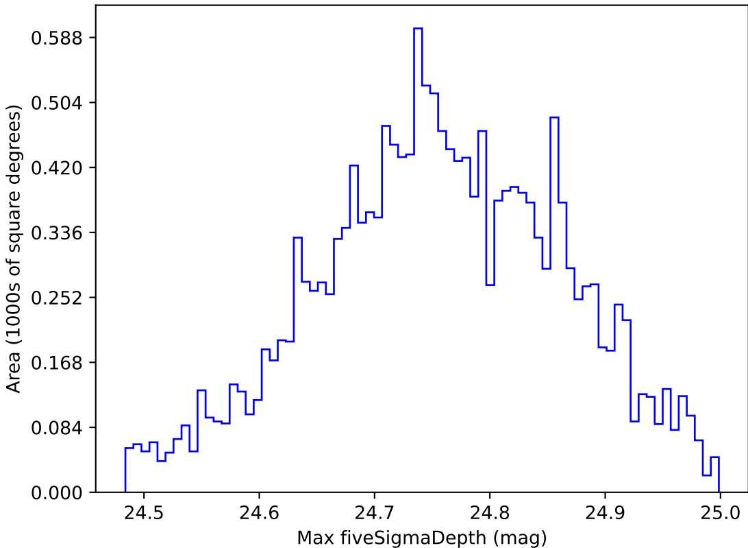
too_elab_r32_d2_gz_v3.4_10yrs WFD r band: Max fiveSigmaDepth
