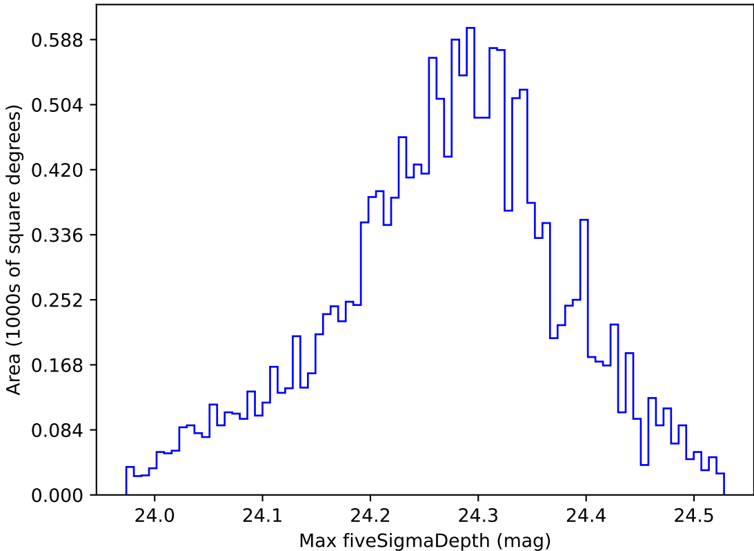
too_elab_r32_d2_gz_v3.4_10yrs WFD i band: Max fiveSigmaDepth
