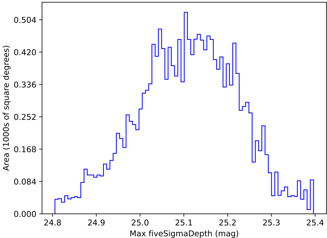
too_elab_r32_d2_gz_v3.4_10yrs WFD g band: Max fiveSigmaDepth
