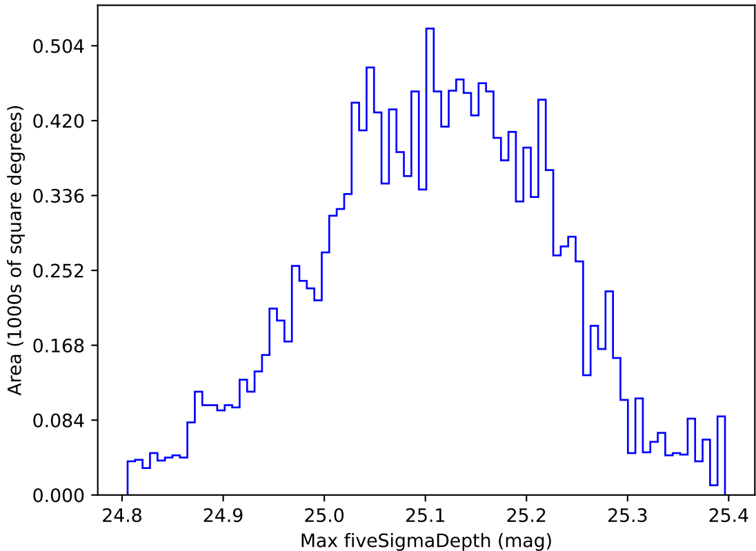
too_elab_r32_d2_gz_v3.4_10yrs WFD all bands: Max fiveSigmaDepth
