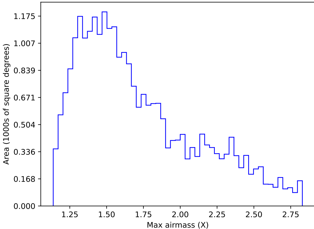
too_elab_r32_d2_gz_v3.4_10yrs Yr 1 z band: Max airmass
