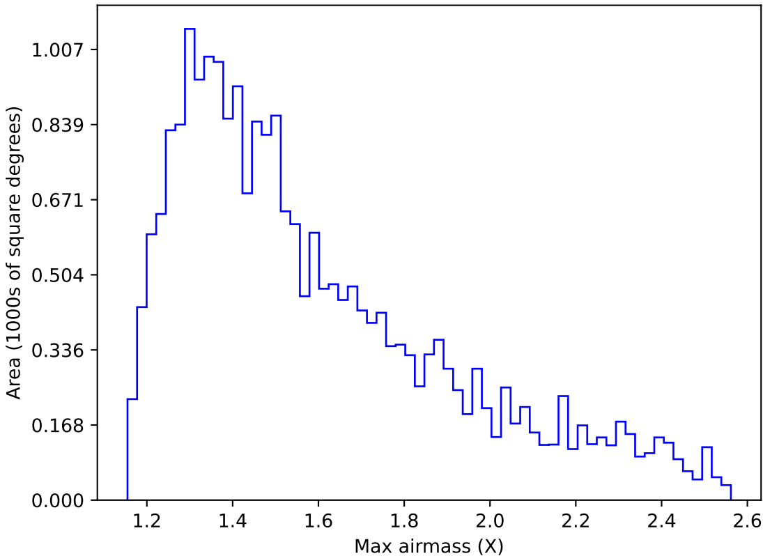
too_elab_r32_d2_gz_v3.4_10yrs Yr 1 y band: Max airmass
