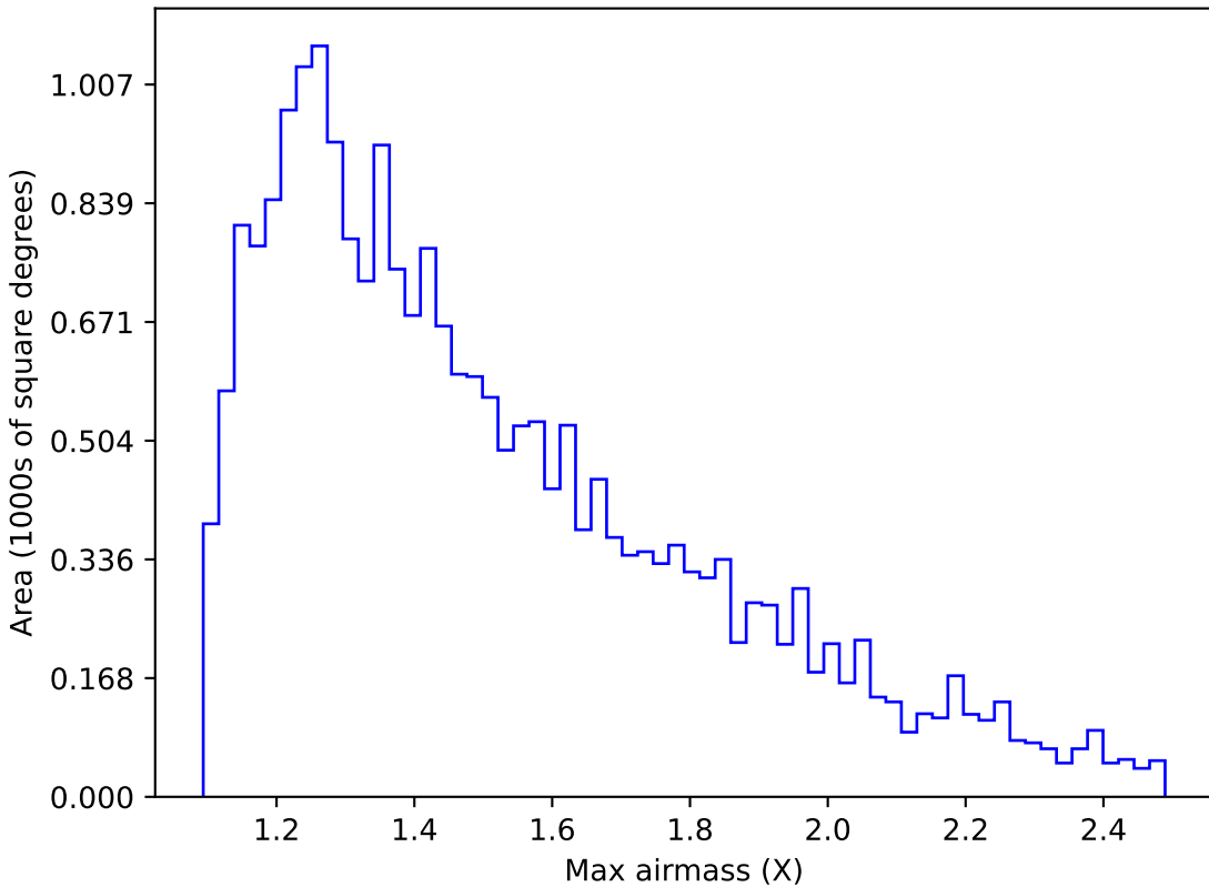
too_elab_r32_d2_gz_v3.4_10yrs Yr 1 u band: Max airmass
