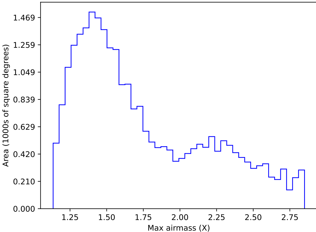
too_elab_r32_d2_gz_v3.4_10yrs Yr 1 i band: Max airmass
