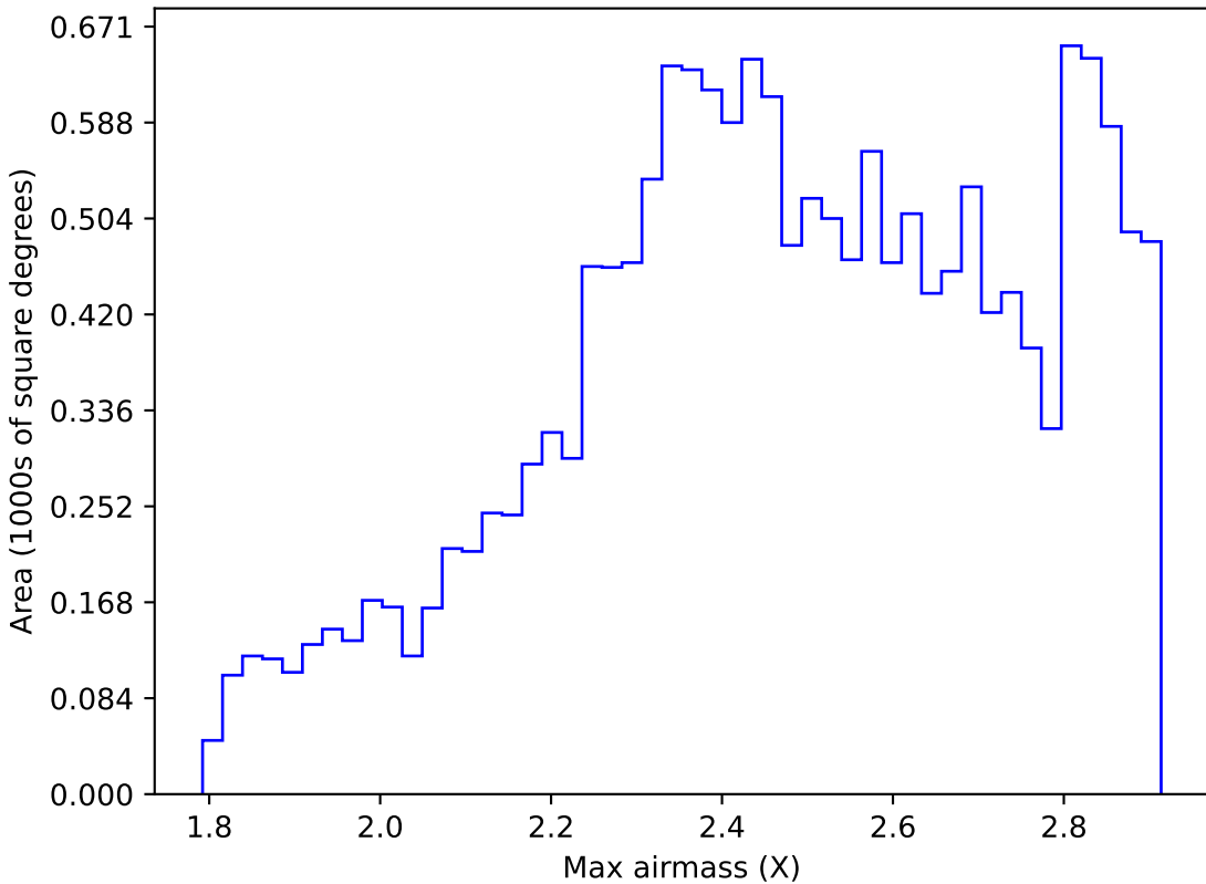
too_elab_r32_d2_gz_v3.4_10yrs WFD z band: Max airmass
