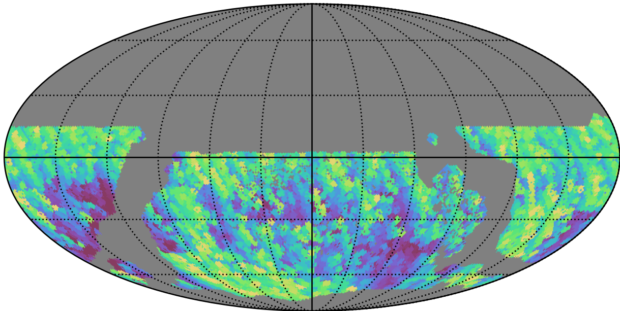
too_elab_r32_d2_gz_v3.4_10yrs WFD y band: Max airmass
