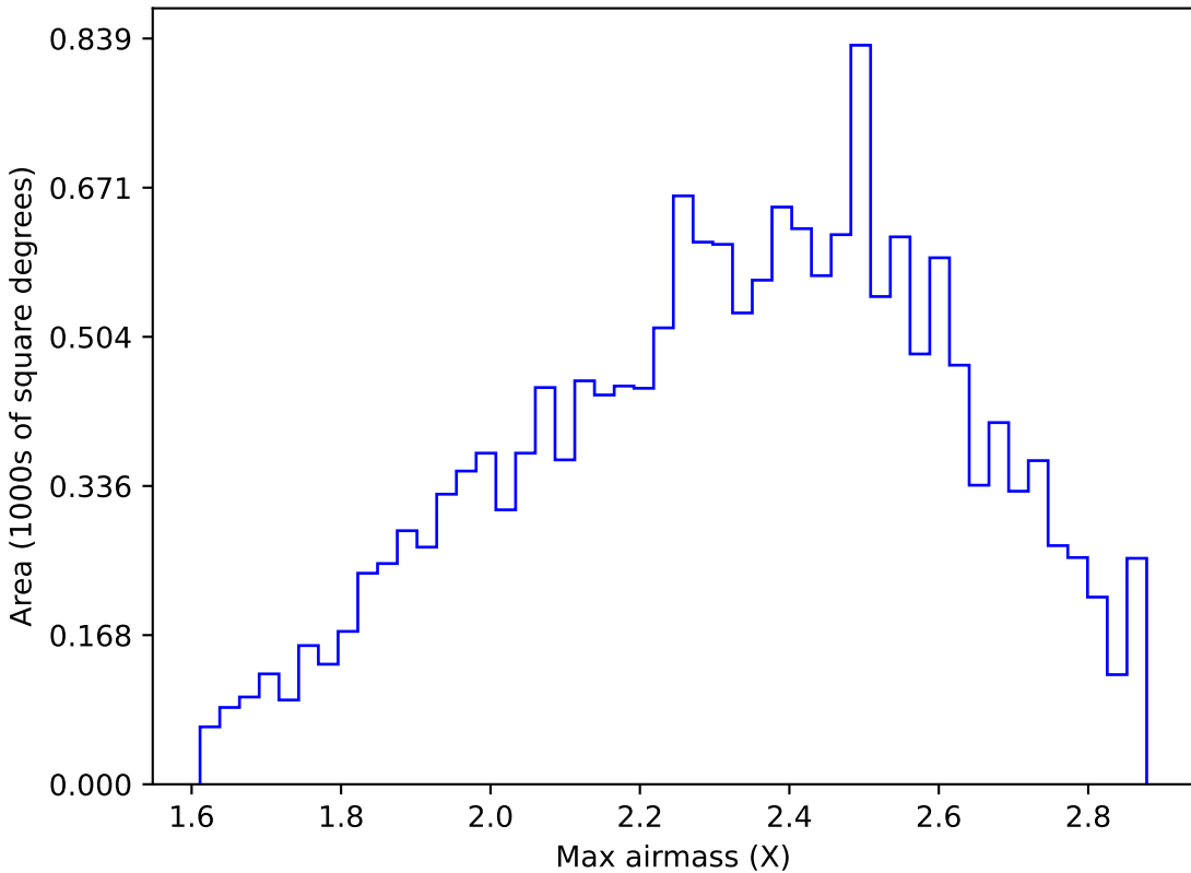
too_elab_r32_d2_gz_v3.4_10yrs WFD y band: Max airmass
