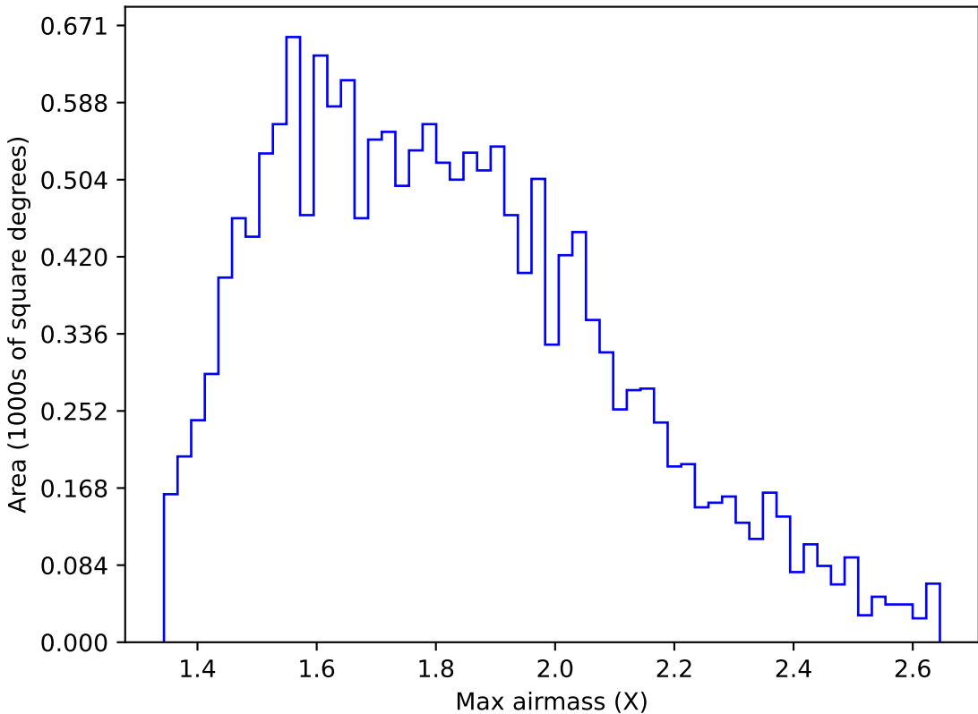
too_elab_r32_d2_gz_v3.4_10yrs WFD u band: Max airmass
