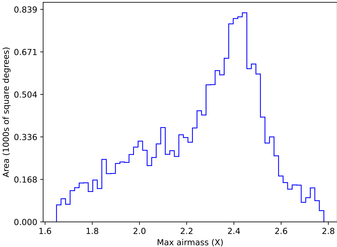
too_elab_r32_d2_gz_v3.4_10yrs WFD r band: Max airmass
