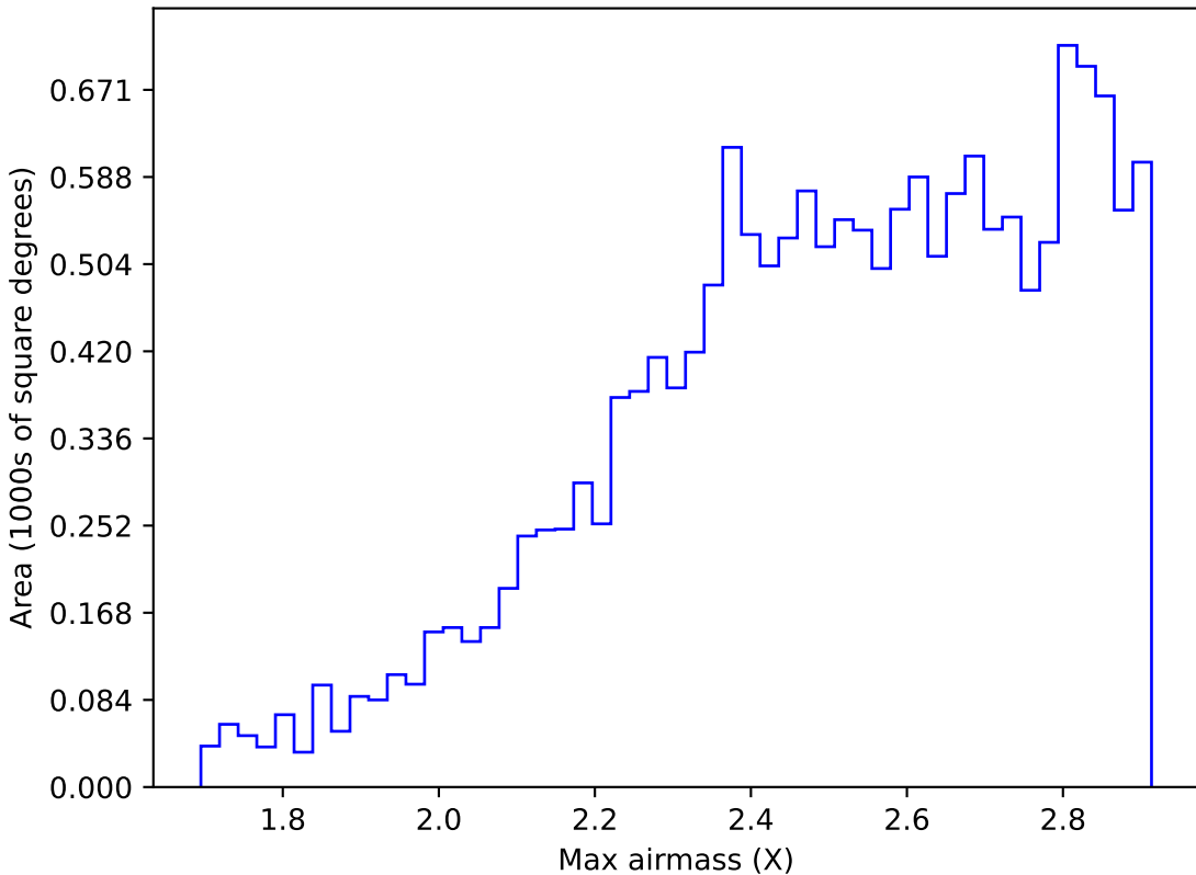
too_elab_r32_d2_gz_v3.4_10yrs WFD i band: Max airmass
