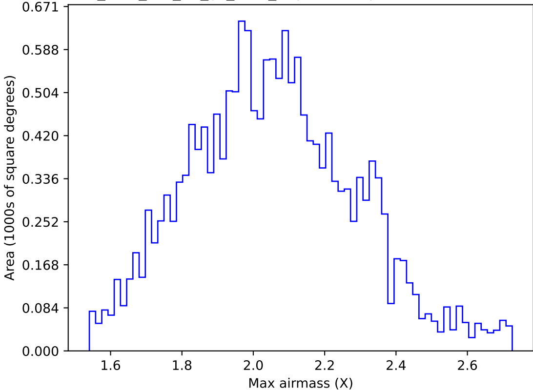
too_elab_r32_d2_gz_v3.4_10yrs WFD g band: Max airmass
