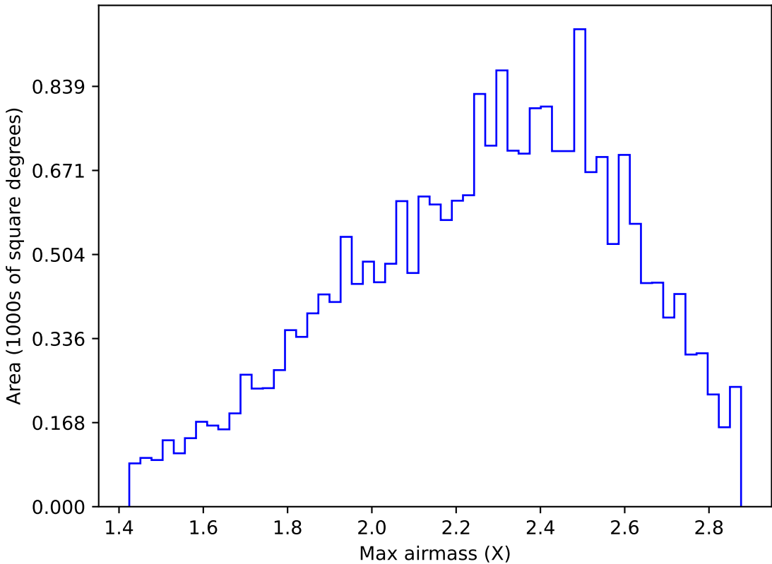
too_elab_r32_d2_gz_v3.4_10yrs All sky y band: Max airmass
