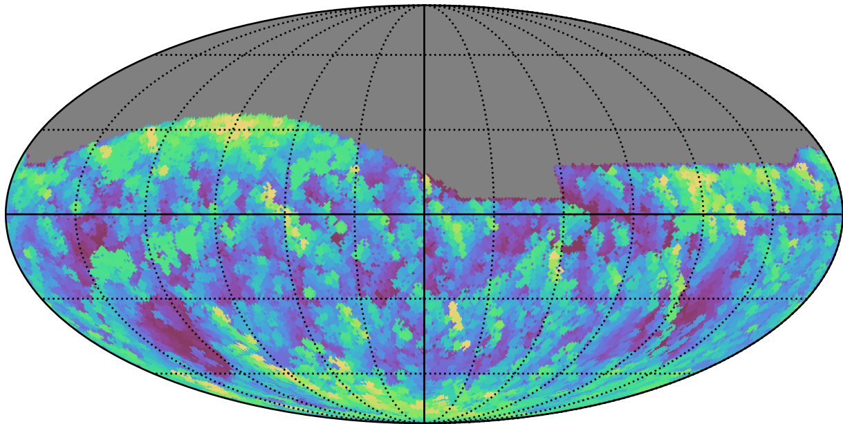
too_elab_r32_d2_gz_v3.4_10yrs All sky g band: Max airmass
